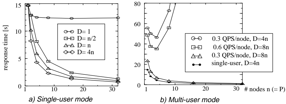
Fig. 6: Performance of non-clustered index scan
