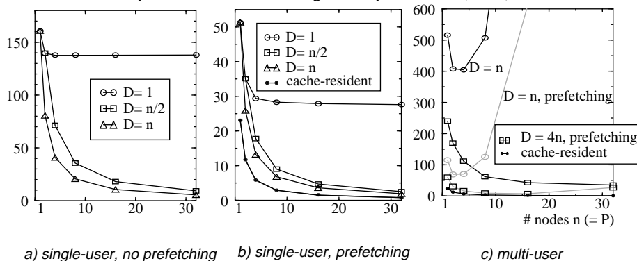
Fig. 4: Performance of relation scan
