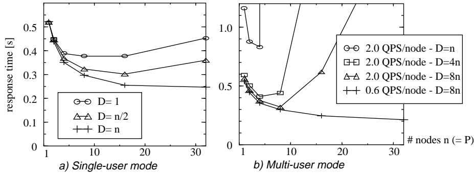
Fig. 5: Performance of clustered index scan
