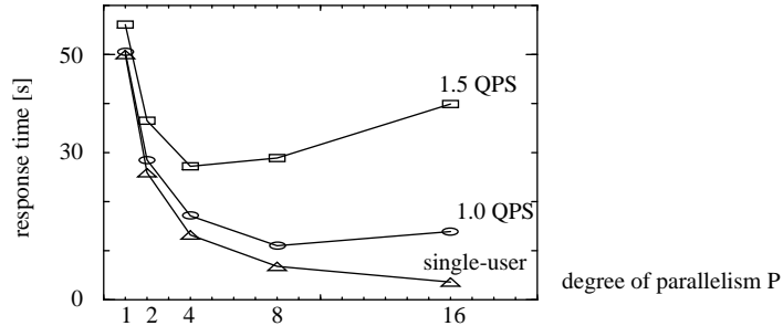
Fig. 7: Degree of parallelism vs. arrival rate ( n=16 , D=64 )
