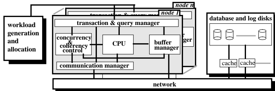
Fig. 2: Structure of the simulation system
