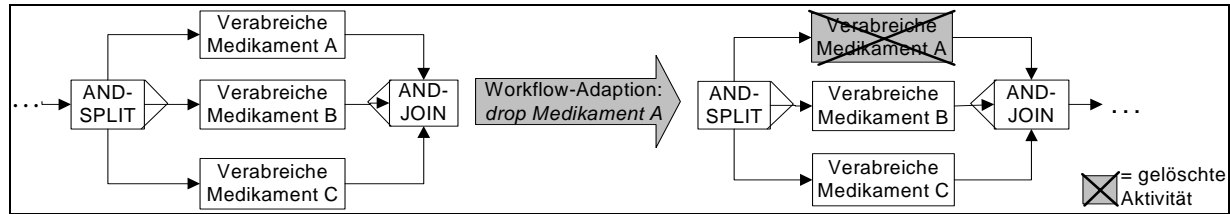
Abb. 2: Workflow-Adaption.
