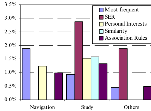
Figure 6: Acceptance rate vs. page type
