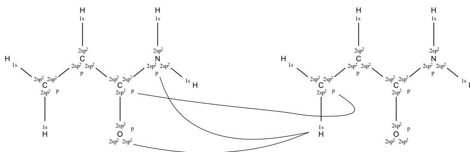
Fig. 2. Selected allowed interactions between two propenamide molecules. The molecules are shown with their atoms surrounded by their valence orbitals. Curved lines indicate some of the allowed interactions: p - p , p - s , and p - l (the sp^2 orbital on O is occupied by a lone pair and thus a l -type orbital).
