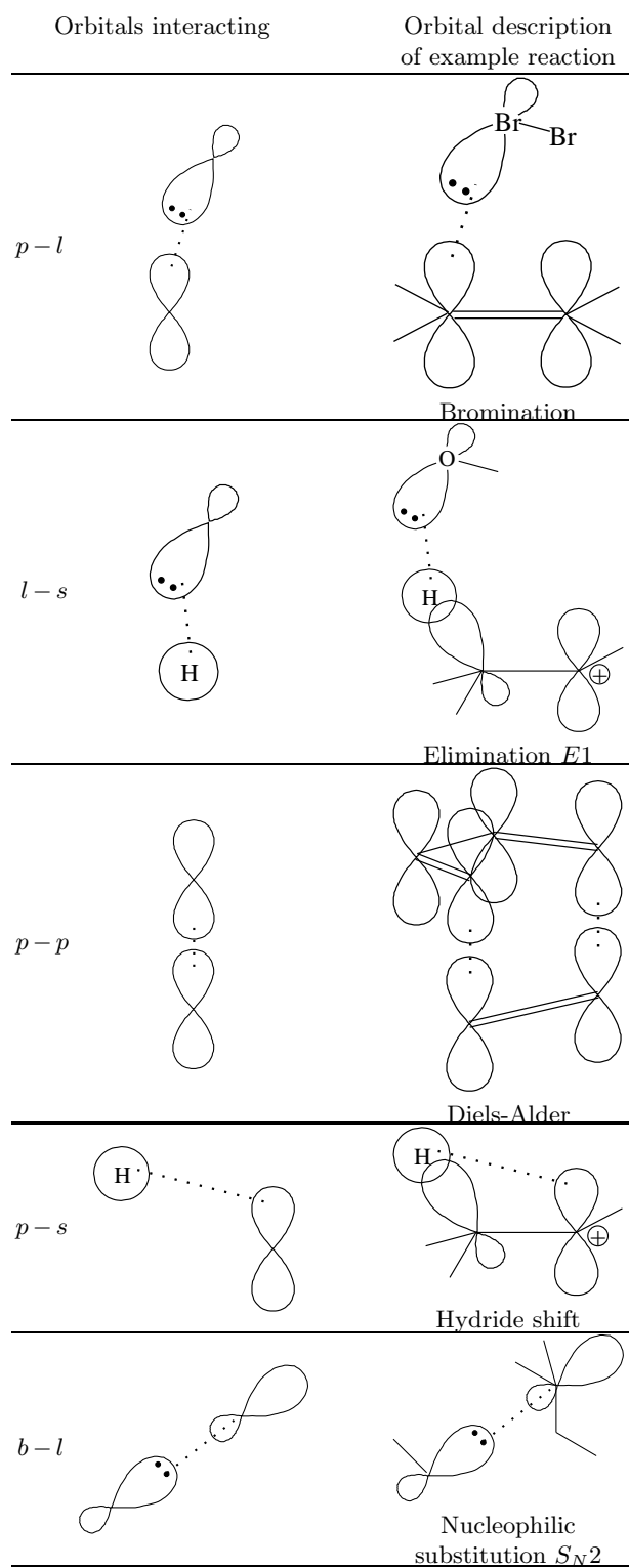
Fig. 1. Allowed interactions. Sketches follow [19].
