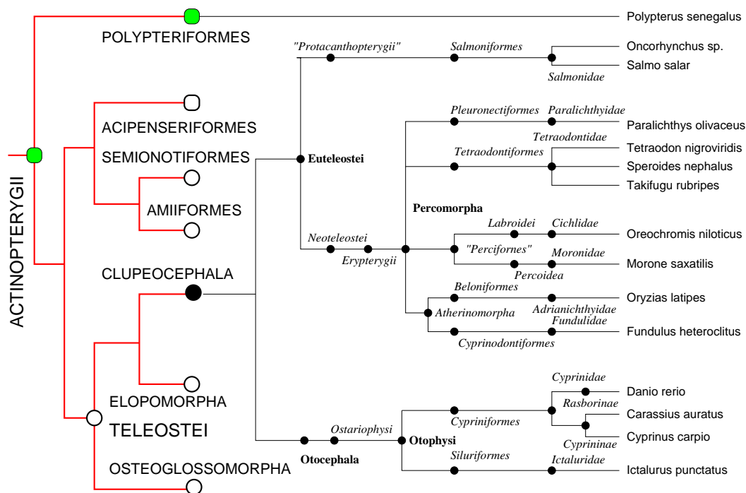
Fig. 1. Phylogenetic relationships among actinopterygian species for which Hox sequences are known. The tree is adapted from a recent extensive survey of mitochondrial genomes [22, 42, 60, 23]. In particular, protacanthopterygii [25] and perciformes [42] seem to be polyphyletic; see also [7] about ambiguities in teleost phylogeny. All investigated clupeocephala have duplicated Hox clusters (see text for references), while the bichir Polypterus senegalus did not share the duplication event(s). [9].
