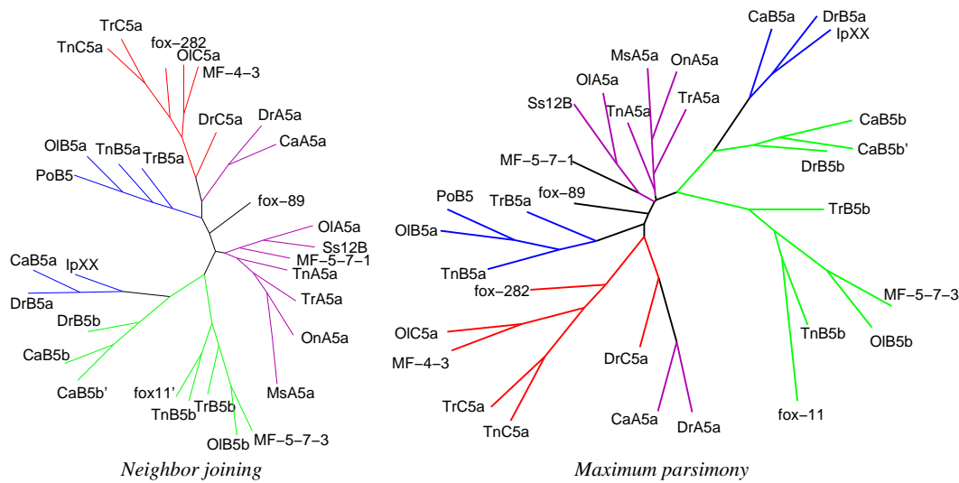
Fig. 3. Reconstructed unrooted trees for homeobox fragments (81nt) for paralog group 5. The tree reasonably identifies the genes in the euteleost and ostariophysii clades. Orthologous genes from within these two groups appear in (phylogenetically reasonable) locations in common subtrees. The resolution of the middle group genes is particularly hard. The weak phylogenetic signal in the 81nt of the homeobox fragments is insufficient to show homology of euteleost and ostariophysii sequences in all cases. MF-5-7-1 and MF-5-7-3 are most likely allelic variants for the medaka genes HoxA5a and HoxB5b . Likewise CaB5b and CaB5b' are allelic variants of the respective goldfish gene.
